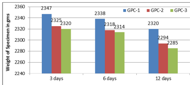
Figure 6 Density of Geopolymer concrete in different days
