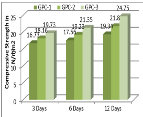
a) Steam Curing
