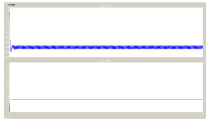
Figure 10 Open Loop Maximum Power Point Input And Output Voltage
