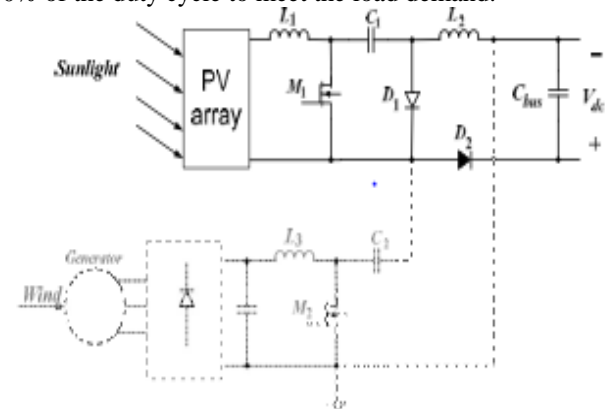
Figure 4 Mode: When M1 Is On And M2 Is Off (Cuk Operation)
