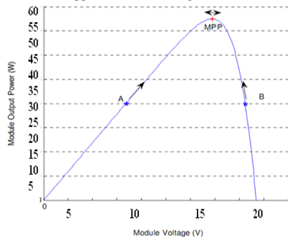
Figure 6 MPP Tracking using P & O Algorithm
