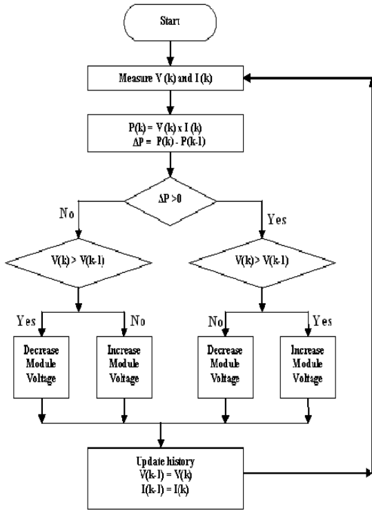
Figure 7 Flowchart of P&O Algorithm
