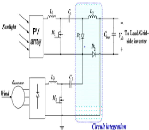
Figure 1 Circuit Diagram
