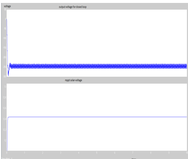
Figure 14 Closed Loop Output with Maximum Power Point Input And Output Waveform
