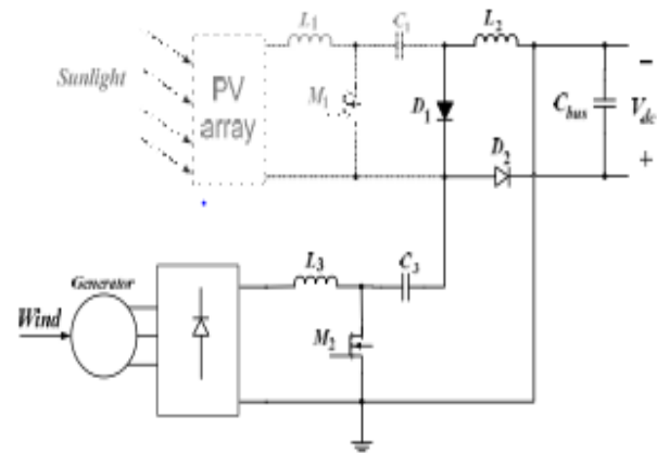
Figure 3 Mode 1: When M2 Is On And M2 Is Off (Sepic Operation)
