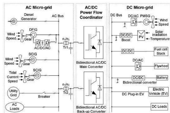
Fig. 1. A Hybrid AC/DC microgrid system
