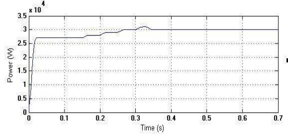
Fig. 9. Output power of the DFIG
