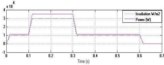
Fig. 5. PV output power versus solar irradiation
