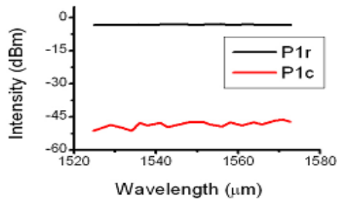
Fig.4. Power Coupled into the Upper port (P1r) when the Optical Beam is steered into the Upper port and the Cross talk at the Lower port (P1c).
