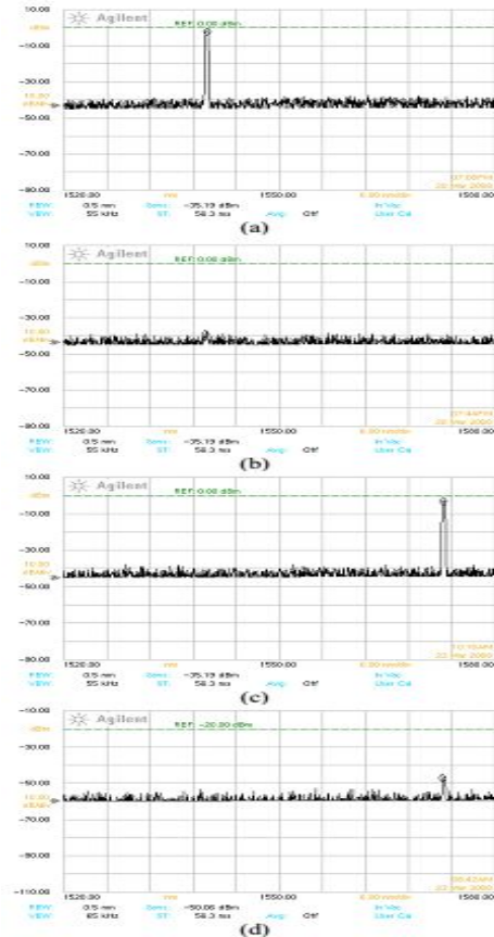
Fig.3.(a) and (c) Maximum Optical Power Coupled Back into Upper port, (b) and (d) Crosstalk at the Lower port. Input Wavelength is 1539 nm for (a) and (b), 1576 nm for (c) and (d).
