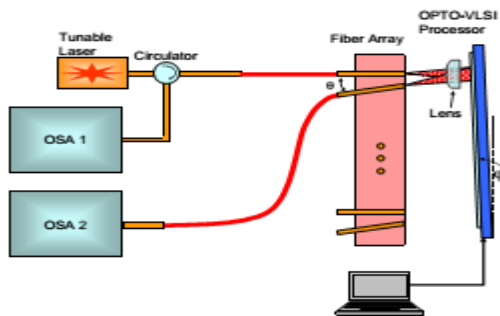
Fig 2. Experimental Setup for Demonstrating the Concept of the ROADM Structure.
