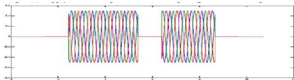
Fig.7 (b) Compensated Voltage injected by DVR for compensating voltage
