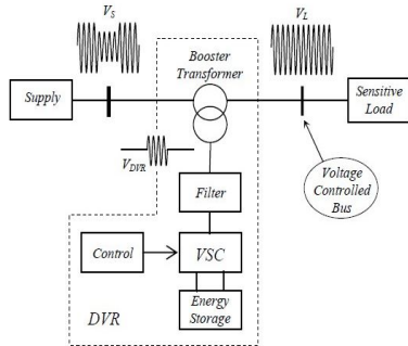
Fig.1 DVR series connected topology The power circuit of the DVR is shown in Fig.1.
