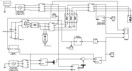
Fig.5 MATLAB model of DVR connected system
