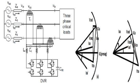
Fig.2 (a) Schematic diagram of DVR Figure-3: Phasor Diagram for (a) Voltage Sag (b) Voltage Swell
