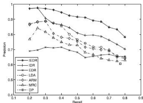
Fig. 3. Comparison of proposed algorithm with existing algorithm for precision-recall curve.
