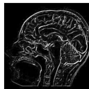
Fig. 15 Resultant image
