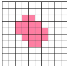
Fig. 3 Dilated image [8]
