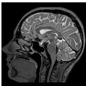
Fig. 8 Original Image
