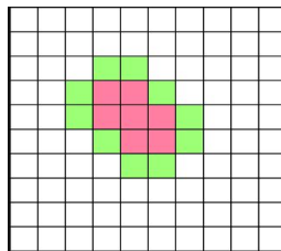
Fig. 2 Applied Mask [8]
