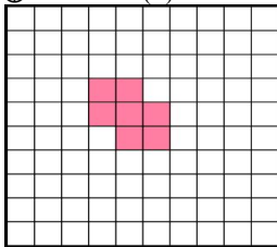
Fig. 1 Original [8]
