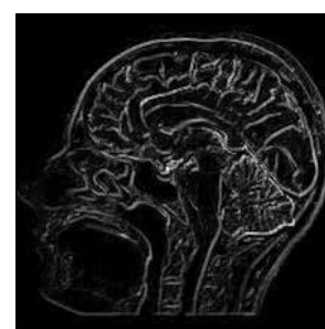
Fig. 12 Closing
