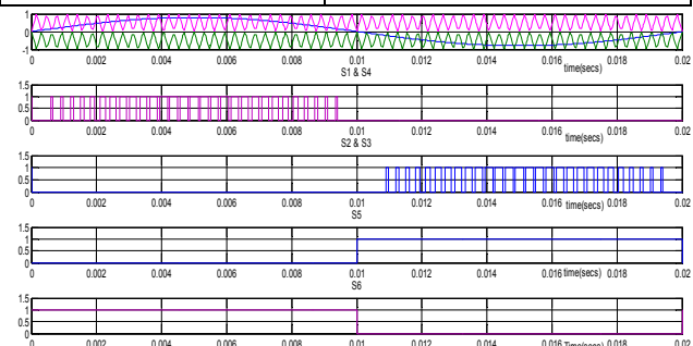
Fig 12. SPWM Waveform- H6 topology
