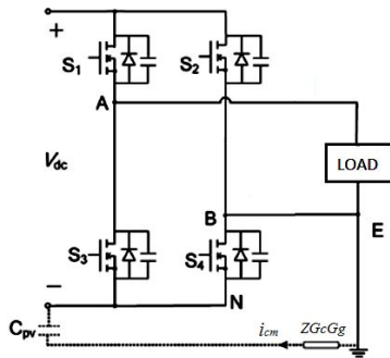
Fig. 1. Leakage current in H4 topology
