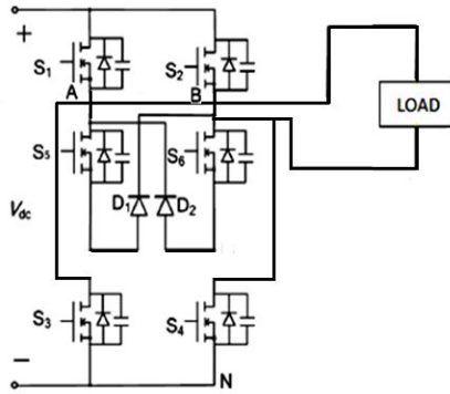
Fig.3. Proposed H6 topology
