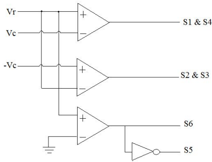
Fig.7. Hybrid modulation
