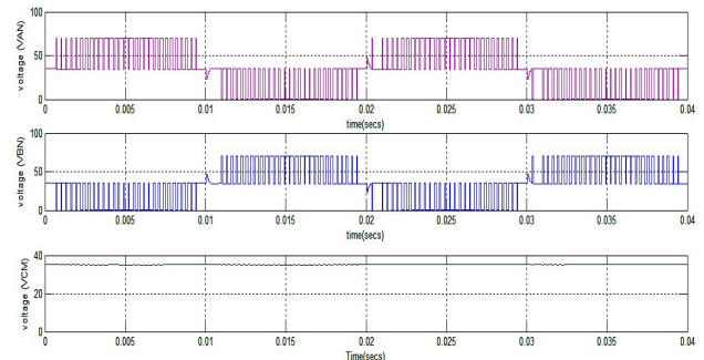
Fig .13. Common mode Voltage of H6 Topology
