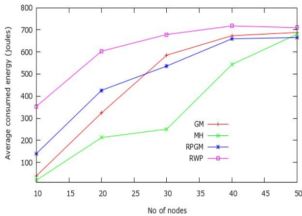
Figure 4.2 Energy Consumption in Receive Mode
