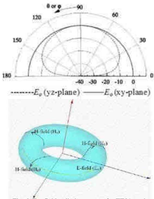
Fig. 6: Far-field radiation pattern for TE 01 mode
