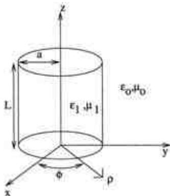
Fig. 4: General Coordinate System for Cylindrical DRA
