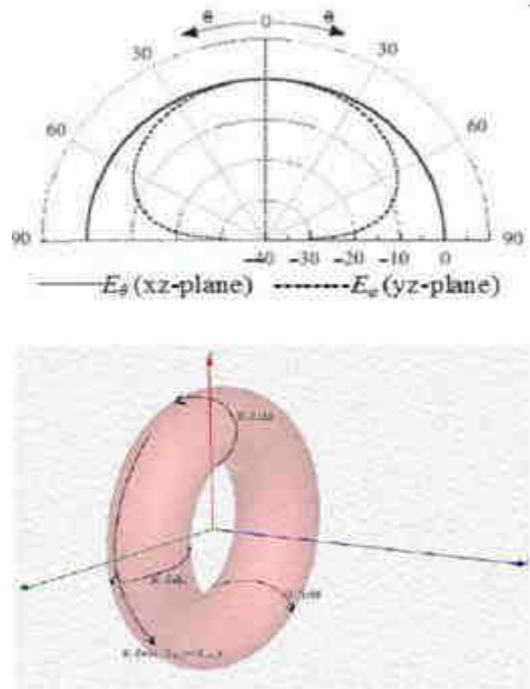
Fig. 8: Far field radiation pattern for HE 11 mode
