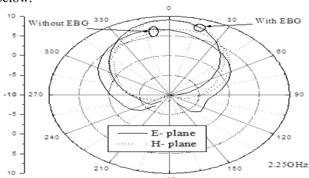
Fig. 13: Radiation Pattern of the DRA
