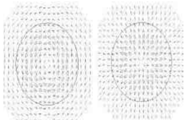
Fig. 1: Mode TE 01 on a dielectric rod waveguide. Left figure shows E-field while Right figure shows H-field
