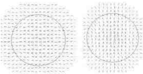
Fig. 3: Mode HEM 11 on a dielectric rod waveguide. Left figure shows E-field while Right figure shows H-field
