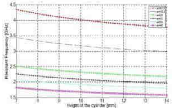
Fig. 9: Resonant frequency as a function of height at different permittivity for TE 01 mode
