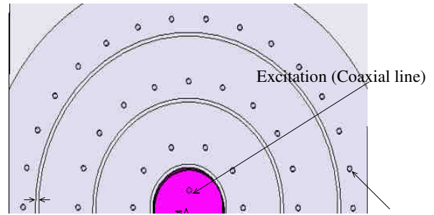
Fig. 12: Graphical representation of DRA design
