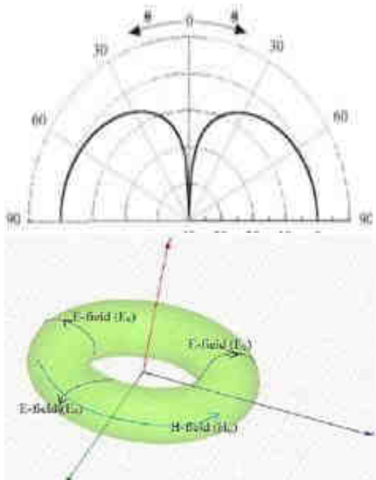
Fig. 7: Far field radiation pattern for TM 01 mode
