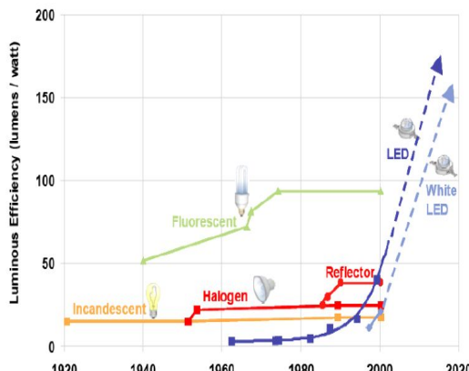
Figure 1. Luminous efficiency timeline for general illumination sources
