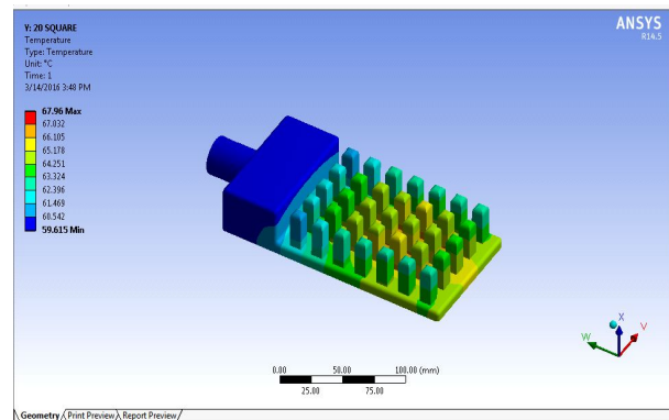
Fig. no.3.2.3 As shown above, after successful run of simulation, found that the maximum temperature reach by base plate by using square 20mm square fins is near about 68° C, and also by using designing software we know the exact weight of this square 20mm finned base plate which is nothing but .70245Kgs.
