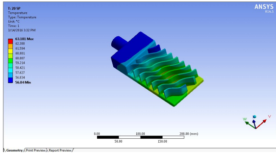
Fig. no.3.2.4 As shown above, after successful run of simulation, found that the maximum temperature reach by base plate by using pline fins is near about 640C, and also by using designing software we know the exact weight of this spline finned base plate which is nothing but .6065 Kgs.
