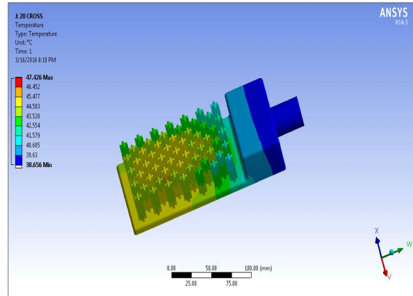
Fig. no.3.2.2 As shown above, after successful run of simulation, found that the maximum temperature reach by base plate by using cross 20mm plus sign fins is near about 47° C, and also by using designing software we know the exact weight of this cross 20mm plus sign finned base plate which is nothing but .66961.Kgs.
